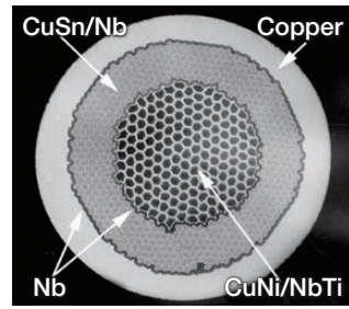
CuNi-NbTi Reinforced
