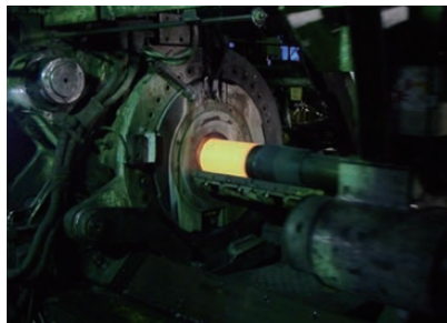
Hot Extrusion
